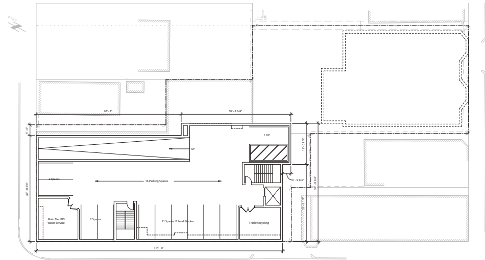
LOWER LEVEL PARKING
